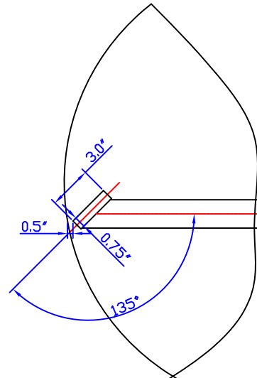
SWEEP BLADE
